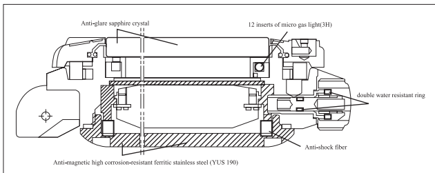
BALL case construction to protect against magnetic fields
